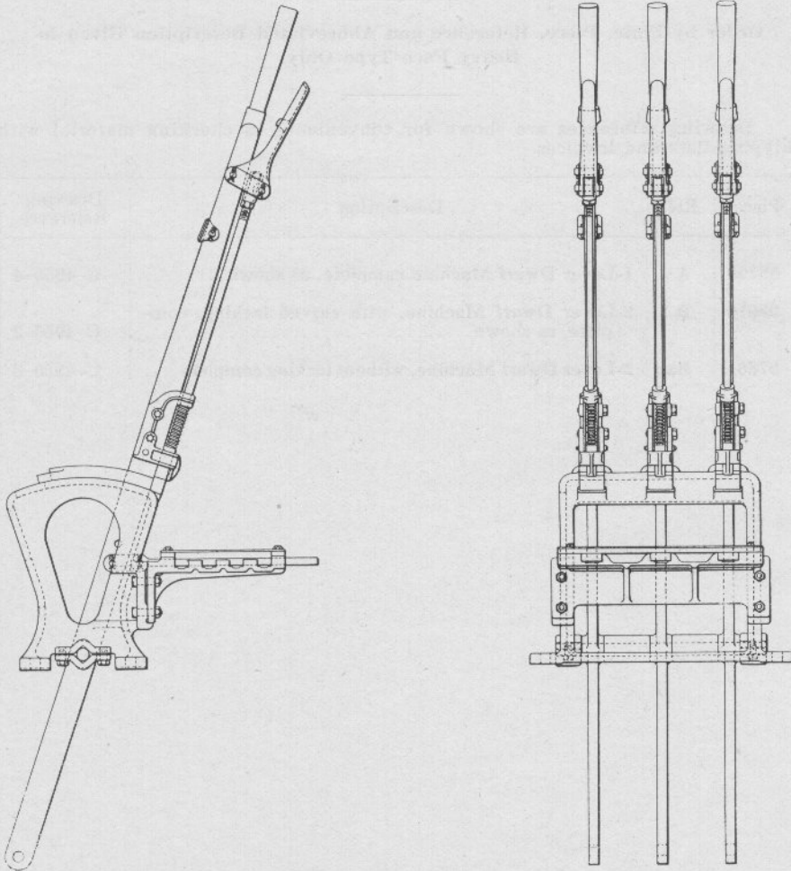
THE DWARF INTERLOCKING MACHINE ARRANGED FOR CONNECTIONS BELOW FLOOR
